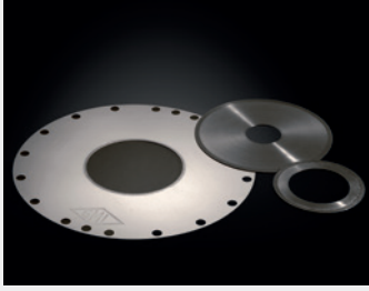
ID Slicing blades are made with natural diamonds to minimize wafer surface and substrate damage.
